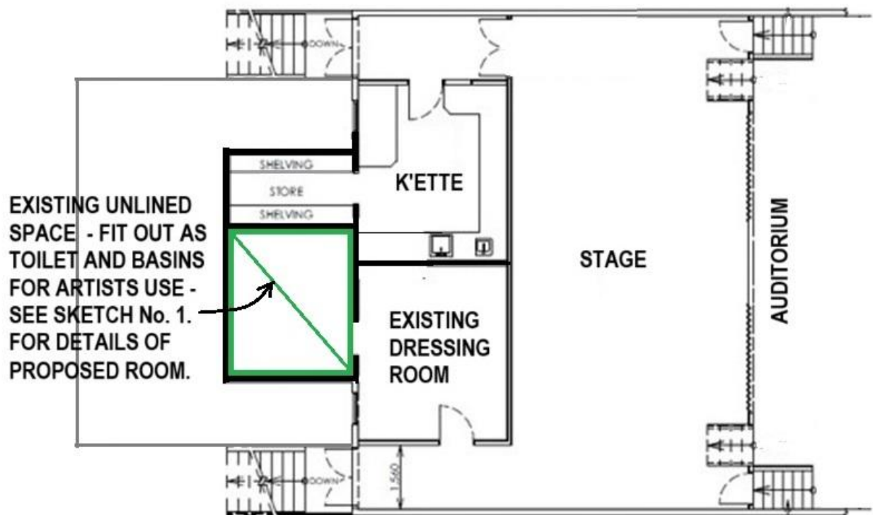
STAGE LEVEL PLAN WITH PROPOSED ARTISTS AMENITIES N.T.S.
